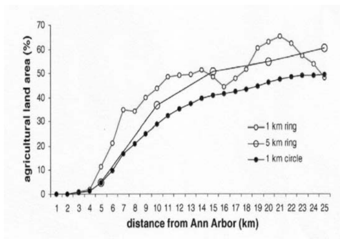
Fig.7. Percentage agricultural land, 1995, calculated using 1 and 5 km rings and 1 km circles.
