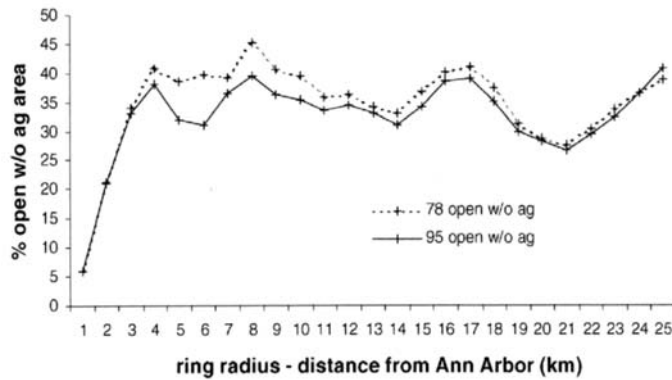
Fig. 5. Percent open space (not including agricultural land), 1978 and 1995, calculated using rings.
