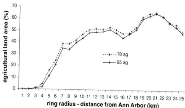
Fig. 4. Percent agricultural land, 1978 and 1995, calculated using rings.
