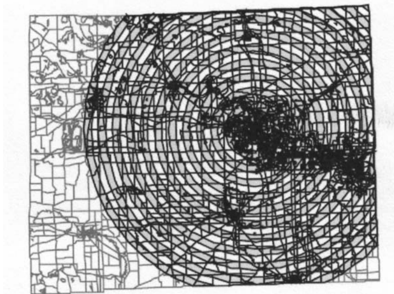
Fig. 3. Example of circles/rings used to generate regional characteristic curves for Washtenaw County, MI superimposed on census block boundaries and centered in downtown Ann Arbor. Increased features and details within a characteristic curve translate into improved function in quantifying and comparing regions.
