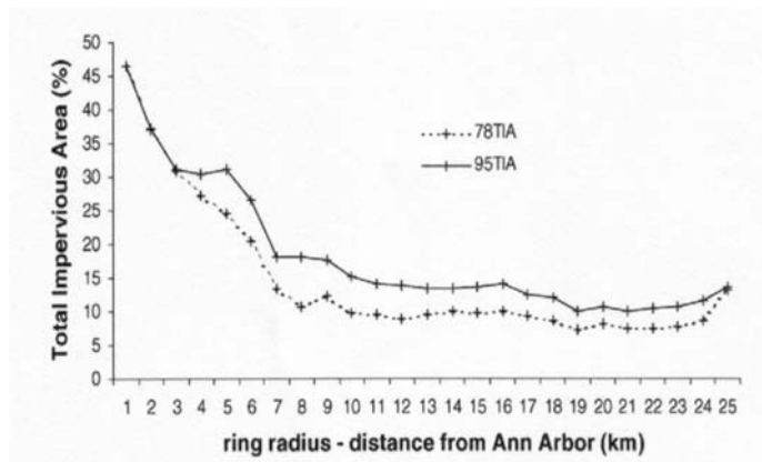
Fig. 6. Percentage total impervious surface area, 1978 and 1995, calculated using rings.
